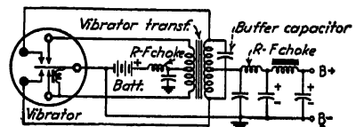
Synchronous vibrator circuit.
